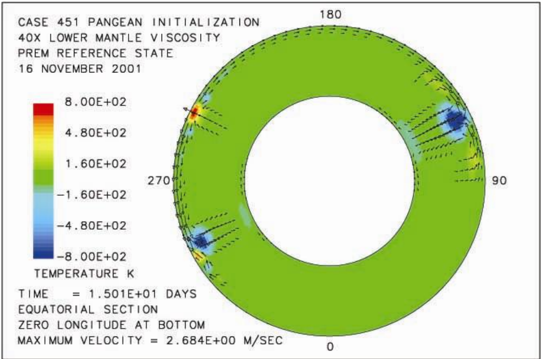
Figure 3(a). Snapshot of 3D solution after 15 days. The upper plot is an equal area projection of a spherical surface 65 km below the top surface in which colors denote absolute temperature. Arrows denote velocities. The dark lines denote plate boundaries where continental crust is present or boundaries between continent and ocean where both exist on the same plate. The lower plot is an equatorial cross section in which the colors denote temperature variation from the mean at a given depth. Arrows denote velocities in the plane of the cross section.
