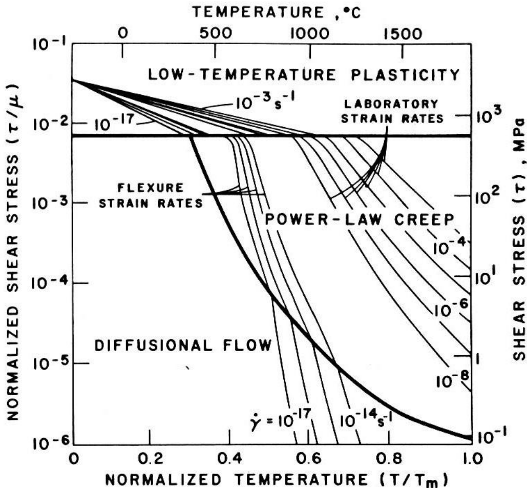
Figure 1. Deformation map for the mineral olivine at 1 mm grain size. Shear strain rates \dot{\gamma} (in s^{-1} ) are plotted versus shear stress \tau normalized by elastic shear modulus \mu and versus absolute temperature T normalized to the melting temperature T_m . [From reference 19 (Kirby, 1983.)]
