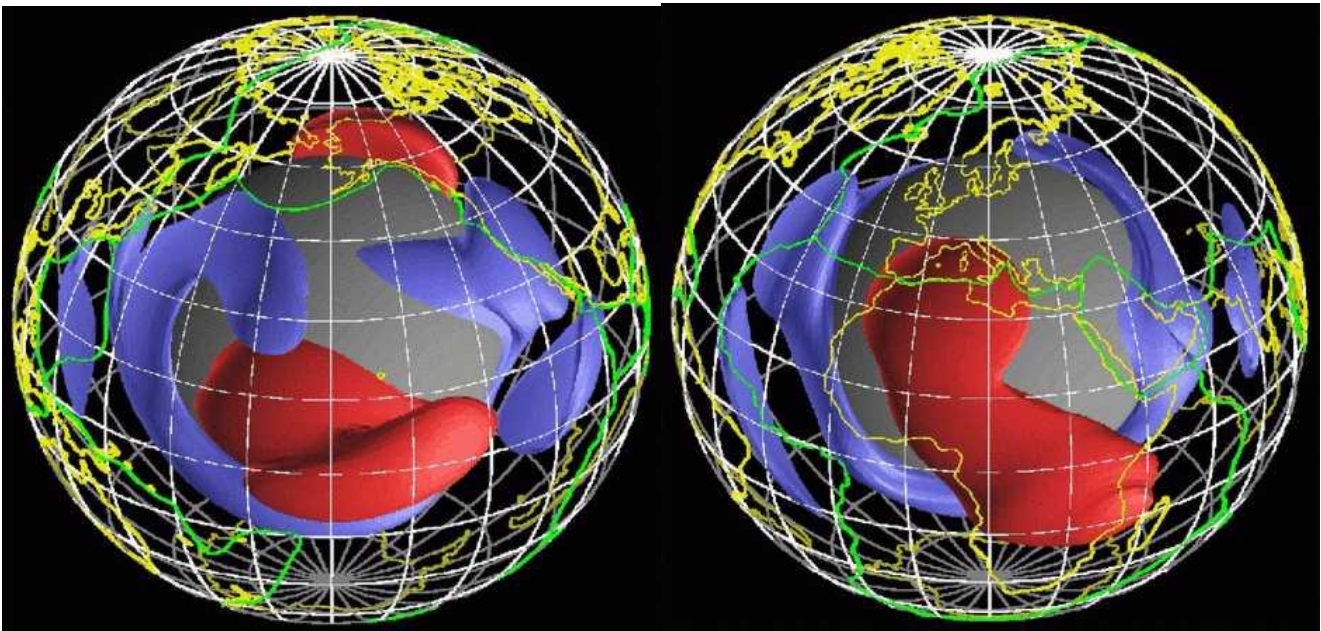
Figure 4. Distribution of hot (red surfaces) and cold (blue surfaces) regions in today's lower mantle as determined observationally by seismic tomography as viewed from (a) 180 degrees longitude and (b) 0 degrees longitude. (Figure courtesy of Alexandro Forte.)
