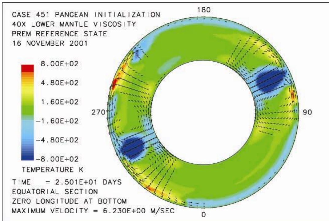
Figure 3(b). Snapshot of the solution after 25 days. Colors and arrows denote the same quantities as in Figure 3(a).
