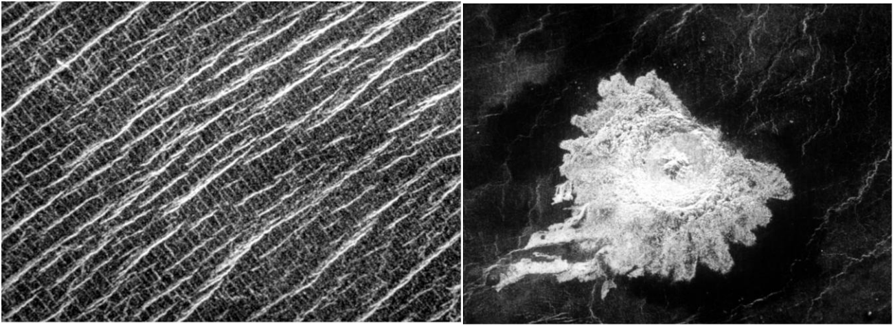
Figure 5. Synthetic aperture radar images of the Venus surface acquired by the NASA Magellan spacecraft. Left image displays the so-called 'gridded plains' terrain associated with massive outpourings of basalt over the planet surface that subsequently cooled and fractured. Right image shows an impact crater about 30 km in diameter whose ejecta blanket is pristine and undisturbed. About 1000 such craters were identified in the Magellan images. The freshness of these craters suggests the tectonism that generated the present Venus surface features was recent. (Images courtesy of NASA Jet Propulsion Laboratory.)
