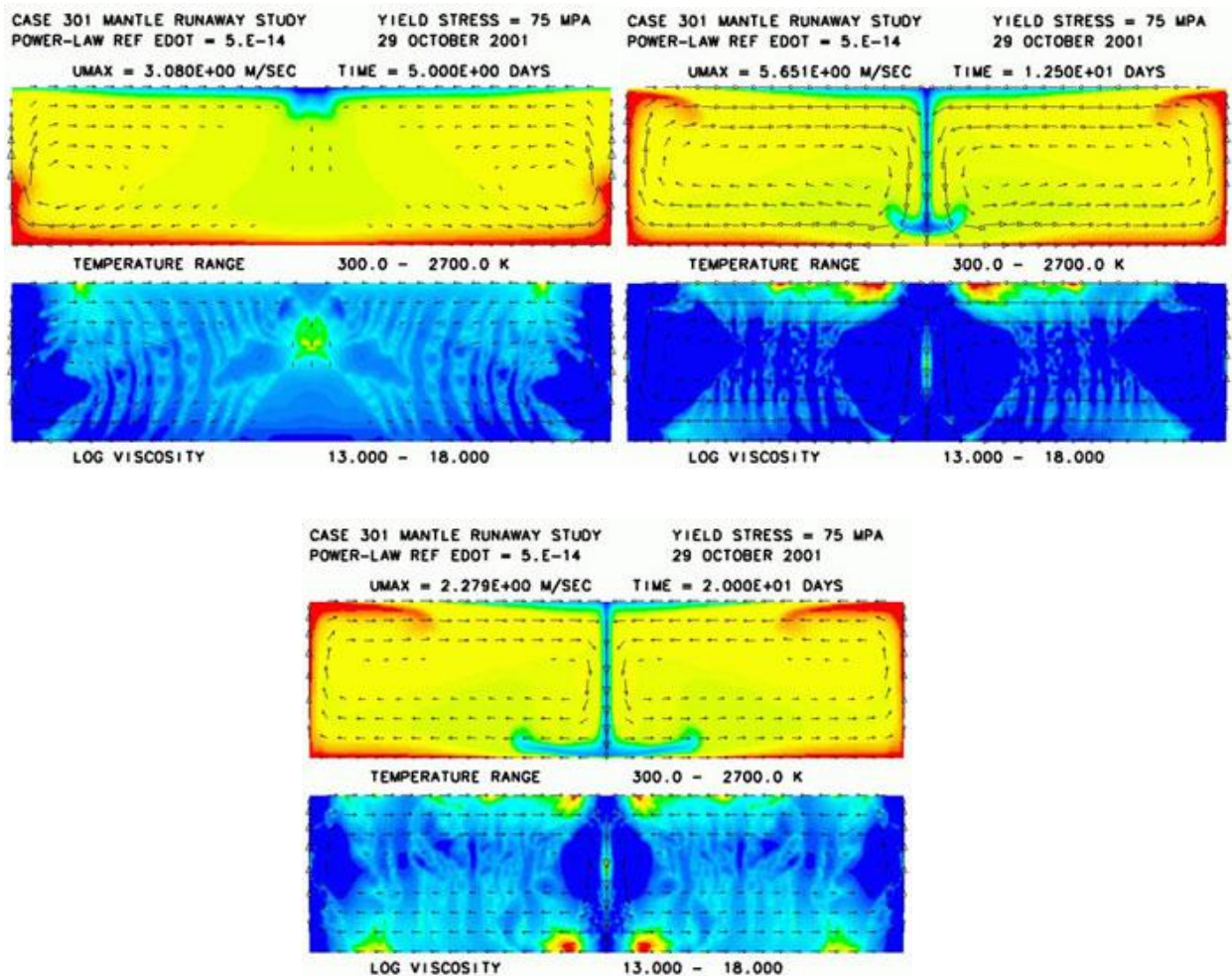
Figure 1. Three snapshots from a 2-D mantle runaway calculation in a box 11,500 km wide by 2,890 km high at problem times of 5, 12.5, and 20 days. Arrows denote flow velocity and are scaled to the peak velocity 'umax'. Contours denote temperatures in the upper panel and base 10 logarithm of viscosity in the lower panel of each frame. Numbers on the contours correspond to a scale from 0 to 10 for the range of values indicated beneath each
